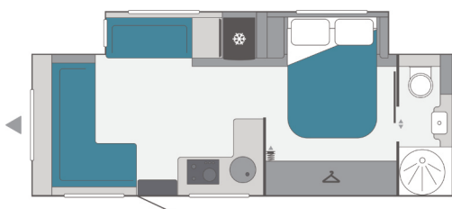
DAY - FLOOR PLAN
