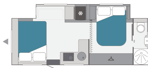
NIGHT - FLOOR PLAN
